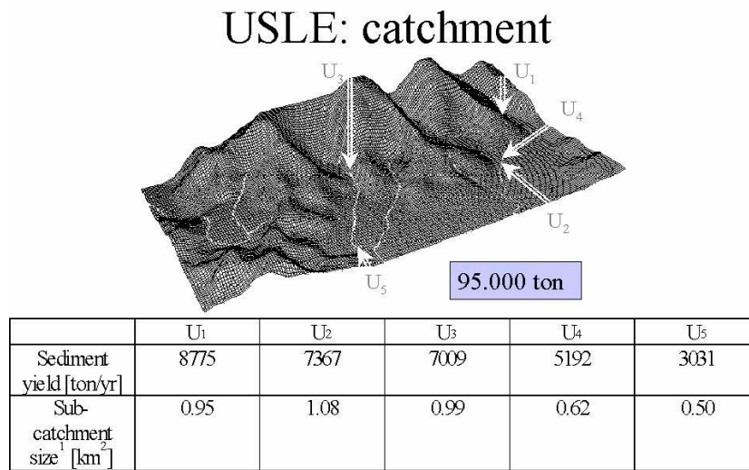
Figure 10. Erosion results and 'hot spots' in a catchment using the USLE for scenario 1. Over the whole grid, the grid cells where sediment would yield are the outer boundaries of the grid and the rivers. These were defined as potential end points for the sediment 'traveling' through the landscape. The five grid cells with the highest sediment yield are listed in figure 10 and 11.
