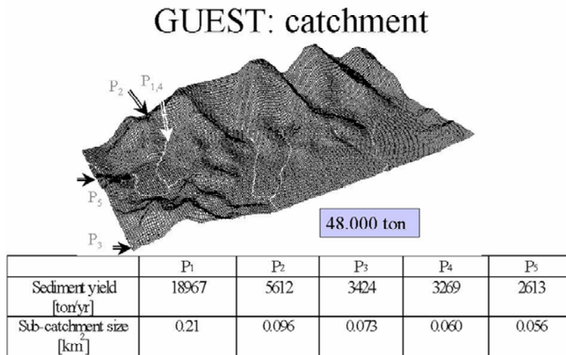
Figure 11 Erosion results and 'hot spots' in a catchment using the GUEST for scenario 1
