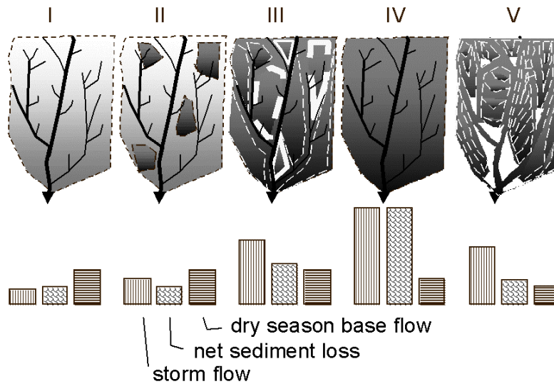
Figure 4. Schematic development of the landscape in a sub-watershed and its effects on storm flow, net sediment loss and dry-season base flow: I. original forest cover, II. patches of forest opened for shifting cultivation, III. intensification of land use has brought most land into cultivation, except for riverine borders and hedges along paths, IV. reclamation of all 'wastelands' has removed all filter strips causing a disproportional rise in net sediment loss, V. restored agroforestry landscape with permanently vegetated contour strips and riparian woodlands.
